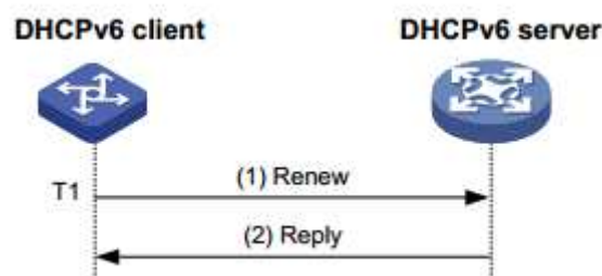
Figure 4: Update address/prefix lease by renew
