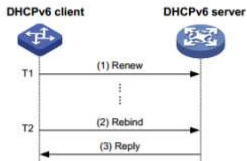
Figure 5: Update address/prefix lease by rebind
